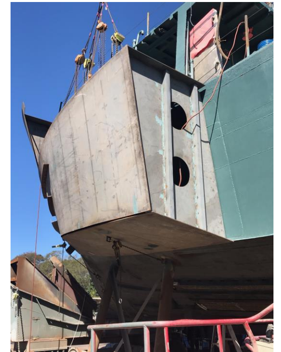
Midship Hull Installed March 12 th
