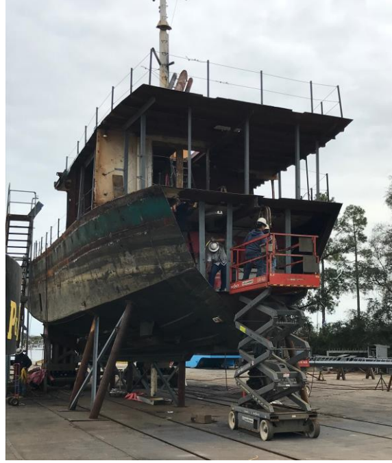
Pilot House, Bow & Focsle Deck Hull Sides Removed February 15 th
