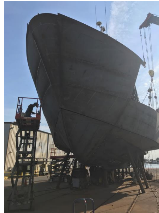
Midship Hull Installed March 12 th
